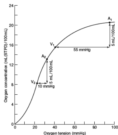
Figure 1: oxygen dissociation curve of whole blood
